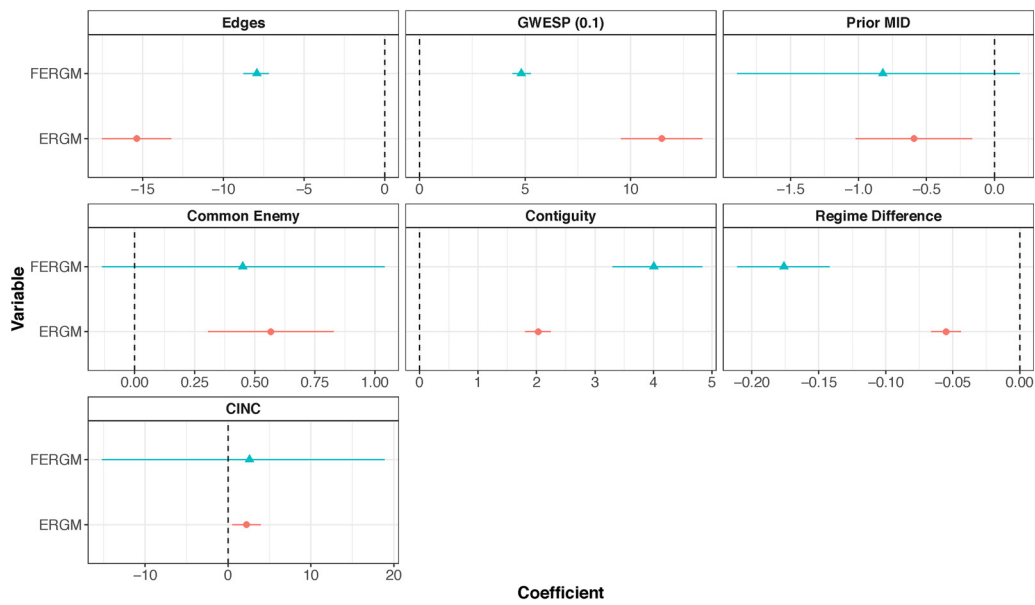
Fig. 6. Coefficient Plot, Alliance Network. 95% confidence intervals presented.
