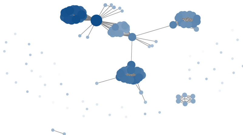
Fig. 5. Defensive Pact Network, 1985. Nodes are sized and colored according to increasing degree.
